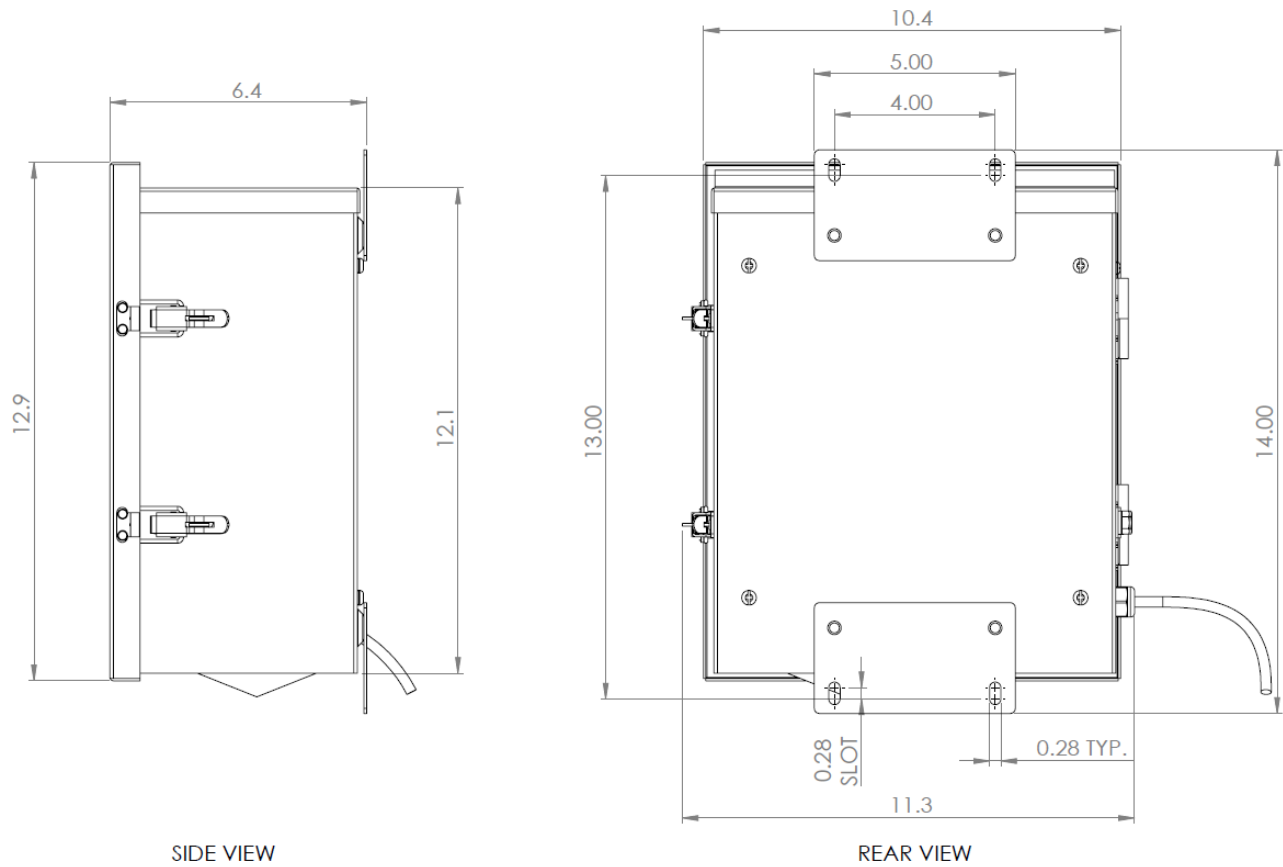
SIDE VIEW
